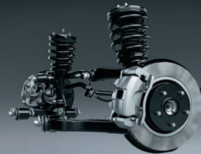
Front double-wishbone – 4x2 suspension shown
