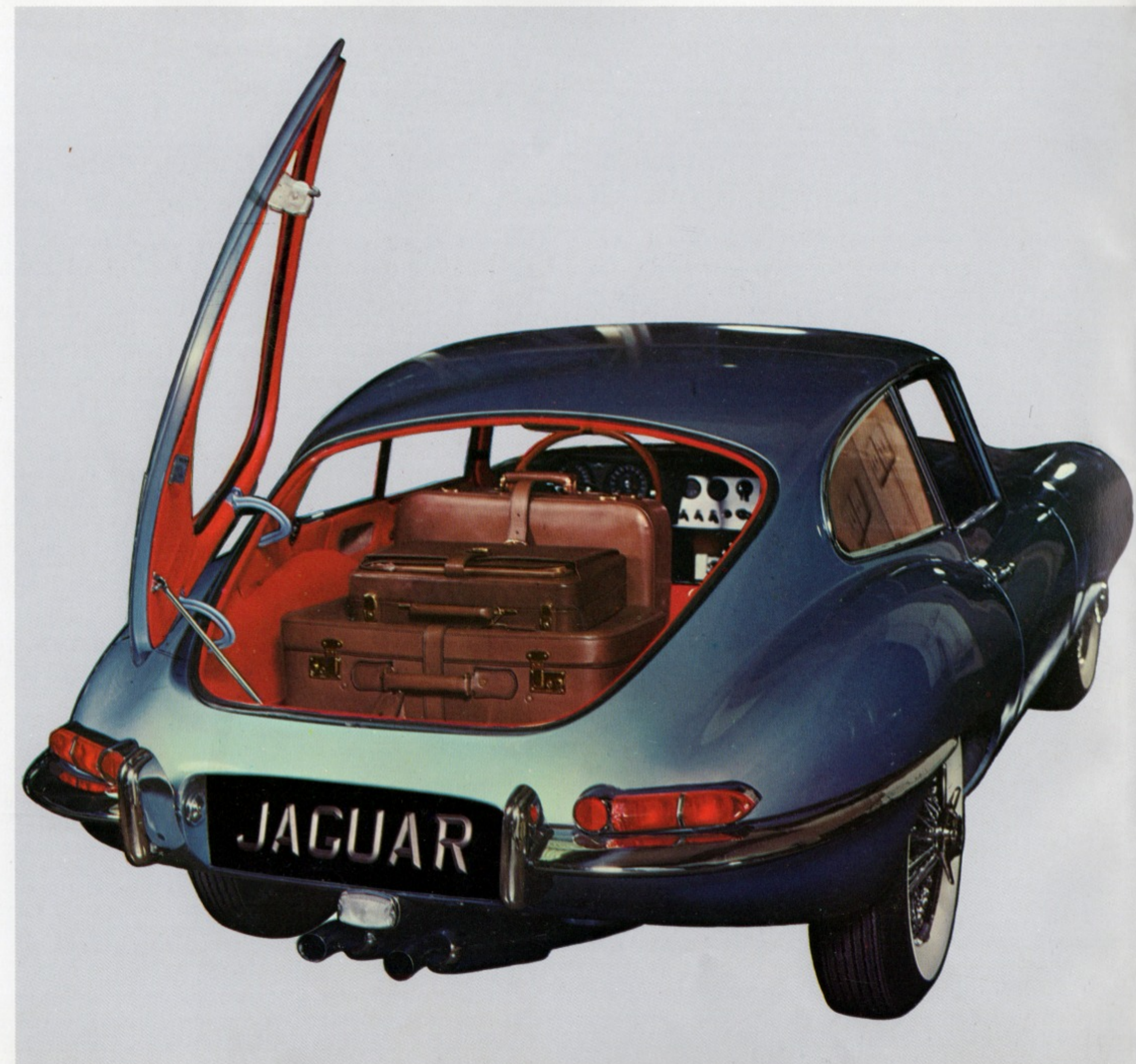
Large counterbalanced door at rear, with release catch located in car, incorporates window and gives unobstructed access to luggage compartment, spare wheel and tools; hinged luggage container behind seats drops down to increase floor space if desired.
