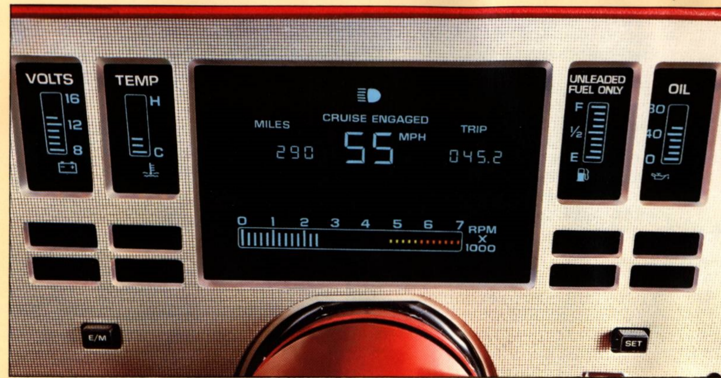
1. Electronic Instrument Cluster. Provides English or Metric Display.
