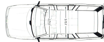
All dimensions are shown in (mm).
