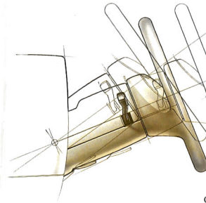
Adjustable steering column for comfort and control.
