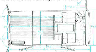
Wheelbase: 90"; Treads: 60" front, 60.2" rear
