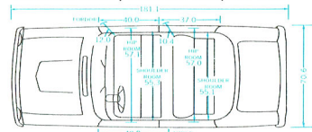
Wheelbase: 109.5"; Treads: 55" front, 54.5" rear
