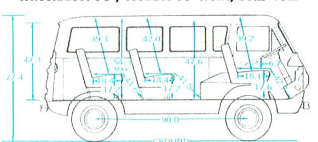
Wheelbase: 90"; Treads: 60" front, 60.2" rear
