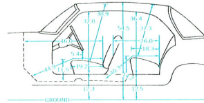
Wheelbase: 109.5"; Treads: 55" front, 54.5" rear
