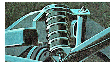
Automatic Load Leveler. Pressurized air bags in each rear spring automatically help keep car at a constant height from the road and level regardless of load.
