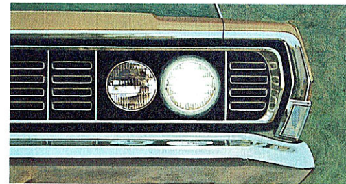
Retractable Headlamp Doors. Dual headlamps are concealed by grille door sections that retract when headlamp switch is turned on. Doors remain closed when parking lights are on. Standard on LTD, XL, Country Squire.
