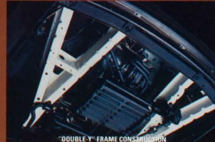
"DOUBLE-Y" FRAME CONSTRUCTION
