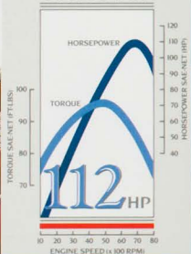
COROLLA GT-S ENGINE MAP
