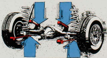
4-LINK REAR SUSPENSION
