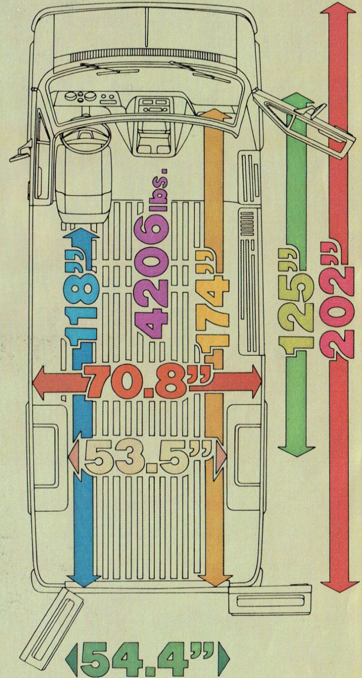
G30, long wheelbase, maximum payload
