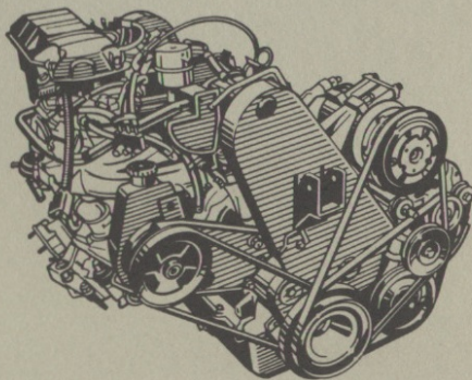
High-Output 2.2-liter OHC engine: 110 hp @ 5,600 rpm; 129 lb-ft torque @ 3,600 rpm.
