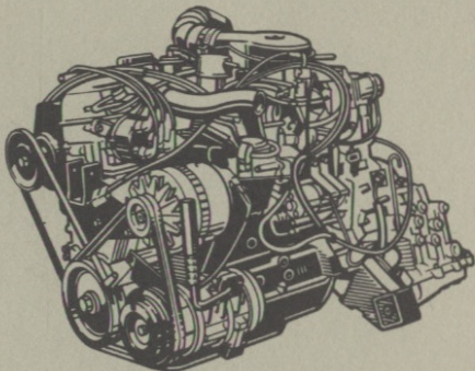
2.6-liter (155.9 CID) four-cylinder engine: 101 hp @ 4,800 rpm; 140 lb-ft torque @ 2,800 rpm. 1
