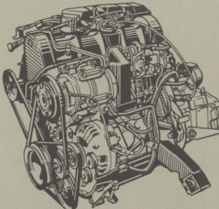
2.2-liter (135 CID) Trans-4 engine: 96 hp @ 5,200 rpm; 119 lb-ft torque @ 3,200 rpm.
