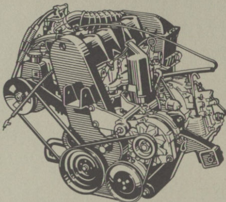
2.2-liter four-cylinder electronically fuel injected engine: 99 hp @ 5,600 rpm; 121 lb-ft torque @ 3,200 rpm.
