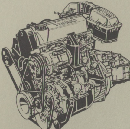
Turbocharged 2.2-liter four-cylinder electronically fuel injected engine: 146 hp @ 5,200 rpm; 168 lb-ft torque @ 3,200 rpm.
