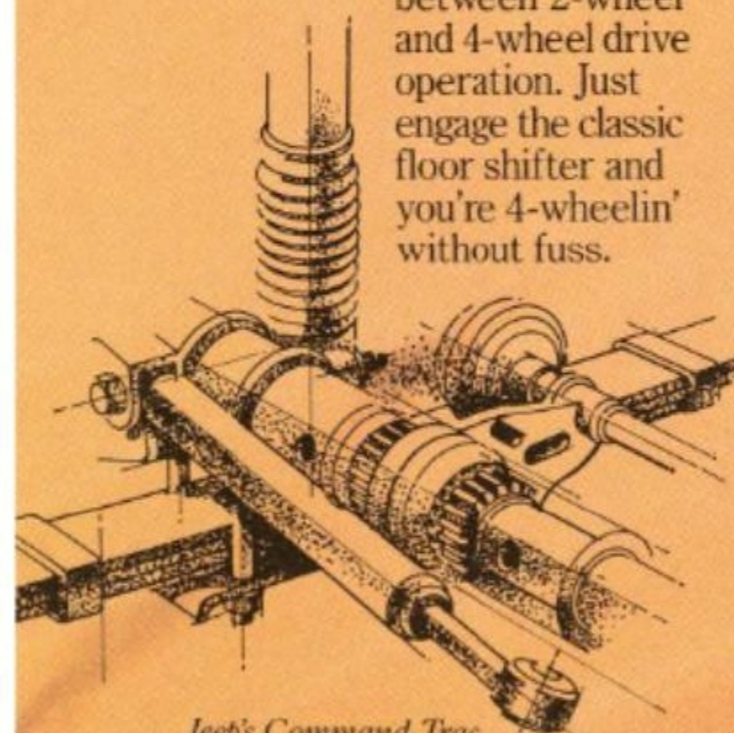
Jeep's Command-Trac 4-wheel drive system lets you shift-on-the-fly between 2WD and 4WD at any speed.
