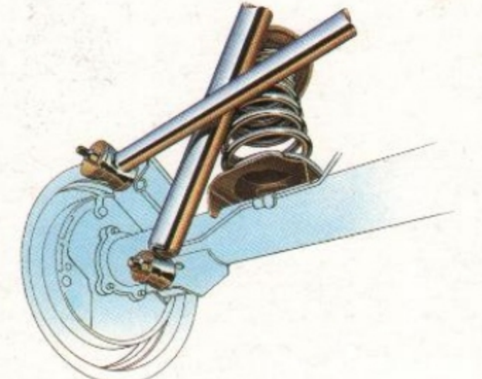
A unique 5-link coil spring rear suspension system has been specially designed to help make the adjustment from highways to byways smooth and easy and to provide greater suspension travel.
