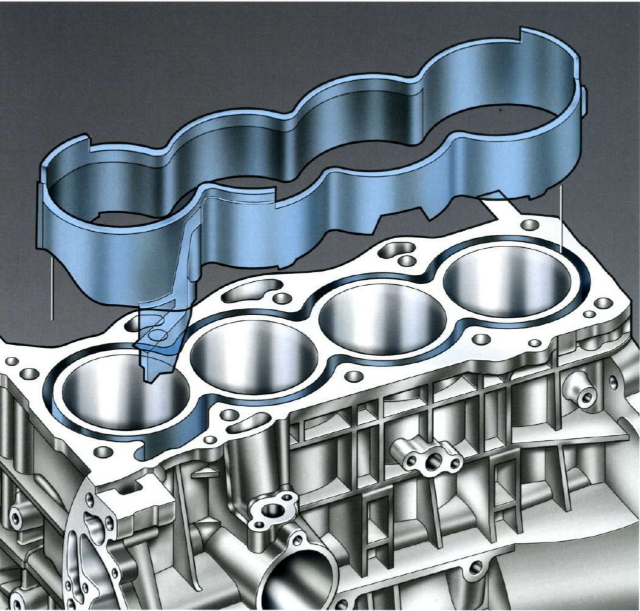
SUPER-COOLING SYSTEM The aluminum-alloy engine uses lightweight, high-compression pistons, kept cool by a "water jacket" that surrounds the cylinder walls. It's a design that also helps make the engine block lighter and more compact.
