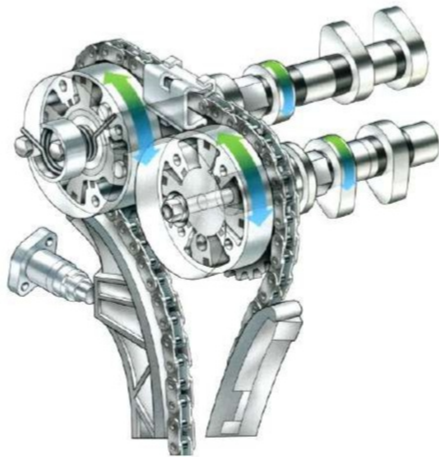
DUAL VARIABLE VALVE TIMING WITH INTELLIGENCE (VVT-i) 2 VVT-i intelligently determines the best valve timing for optimum power and efficiency.
