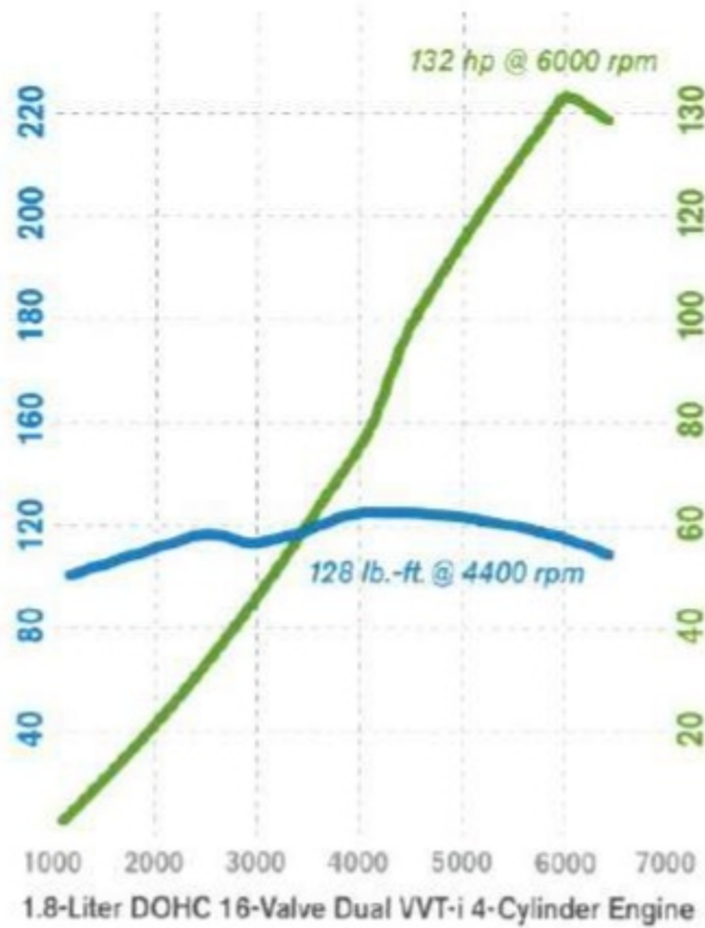
ENGINE POWER Corolla is ready for its debut. Equipped with a highly refined 1.8-liter 16-valve 4-cylinder engine, the engine is rated at 132 hp and 128 lb.-ft. of torque. Proving it doesn't take big bucks to get real bang for your buck.
